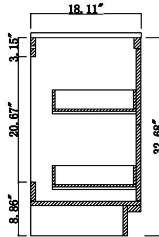
Left View
